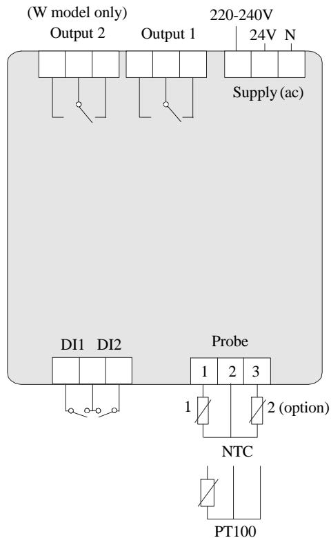
IRDRV & W NB: IRDRTE does not have 24V supply
